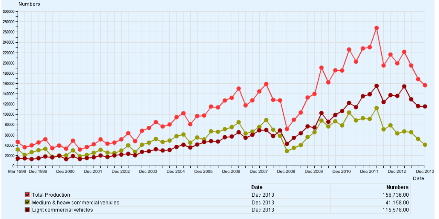
Category-wise Production of Commercial Vehicles : Numbers : Mar 1999 to Dec 2013
